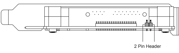
2 Pin Header
